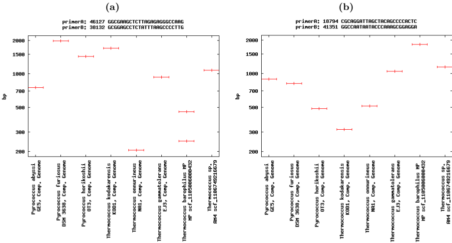
Fig. 4. (a) A randomly chosen theoretical PCR obtained on the studied set of genomes using a pair of primers respecting conditions min = 200 , max = 2000 , limit = 3500 , \delta = 1.10 and max\_occ. = 2 . (b) theoretical PCR obtained on a primer pair respecting conditions min = 200 , max = 2000 , limit = 3500 , \delta = 1.05 and max\_occ. = 1 and defining a variable marker region and a homologous flanking region between set of genomes.
